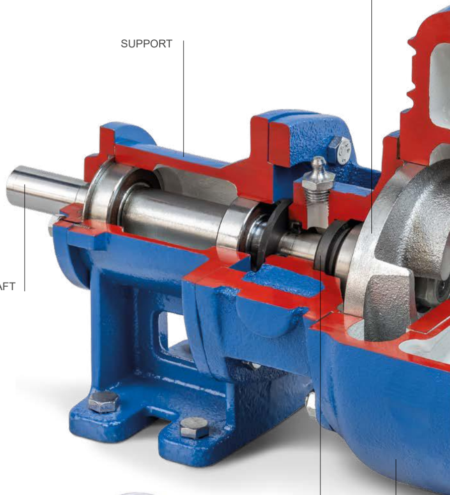
MECHANICAL SEAL
