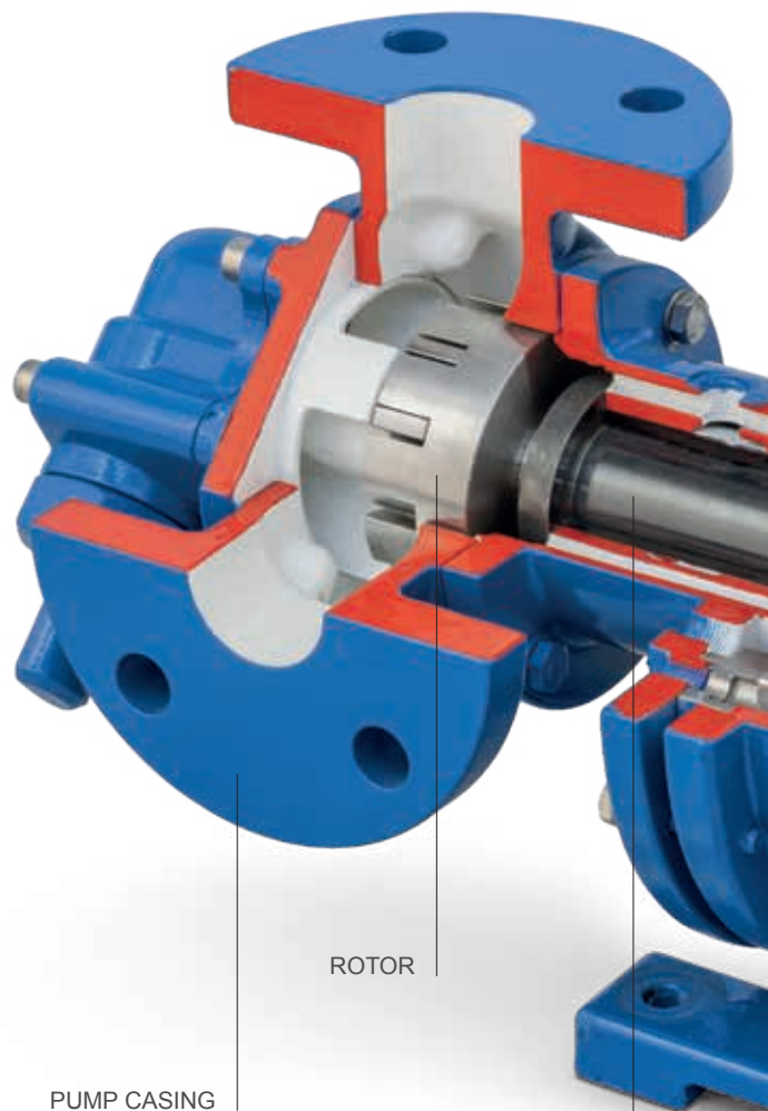
PUMP CASING
